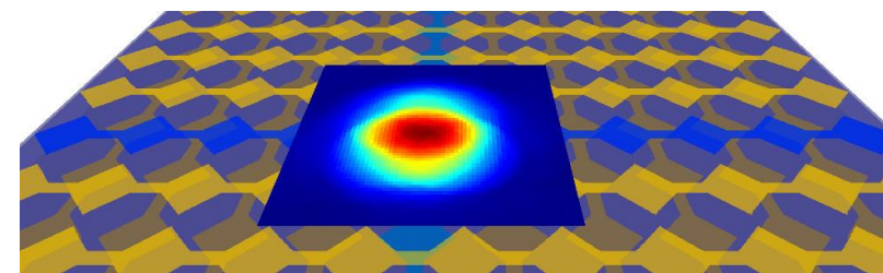
Sensitivity of a mutual capacitance touch surface as simulated in CapExt
