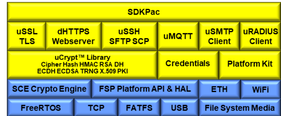
SDKPAC Modular Solution Block Diagram
