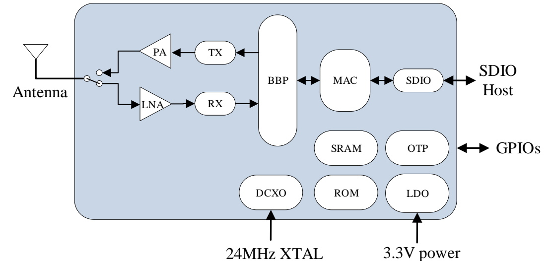
Altobeam Wi-Fi Chip/Module Block Diagram
